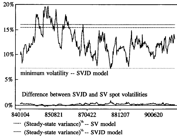
Figure 1 Instantaneous conditional (spot) volatility implicit in deutsche mark options, 1984–1991 Spot volatility is defined as (V_{jump} + V_c)^{1/2} , where V_{jump} is the variance attributable to the time-invariant jump component. The steady-state variance is V_{jump} + \alpha/\beta^* . Expected average variances (roughly the Black-Scholes implied variances) are a maturity-dependent weighted average of spot and steady-state variances.
